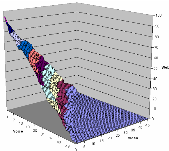
Figure 4: UTRAN Capacity Surface
